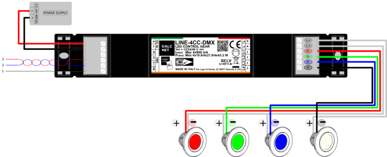
Figure 5: Wiring diagram for RGBW LED load
